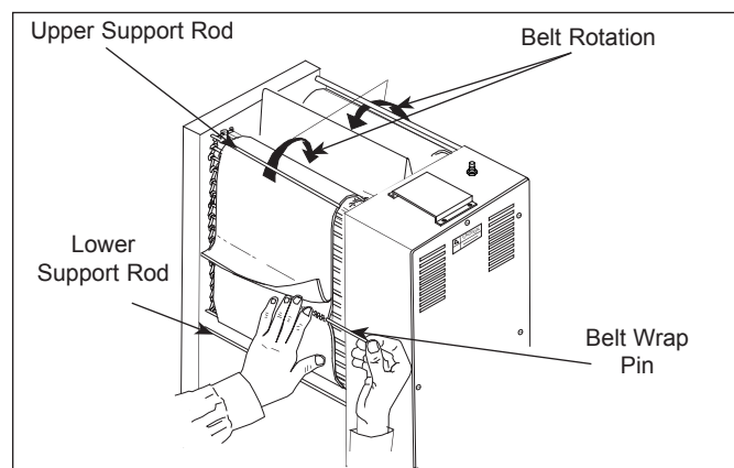
Figure 12. Installing Belt Wrap
